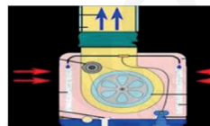
Convection in gases
